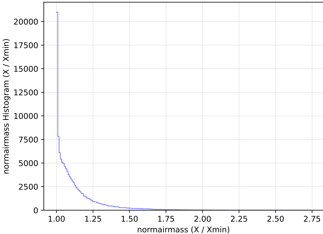
ddf_half_v3.4_10yrs All sky u band: normairmass Histogram
