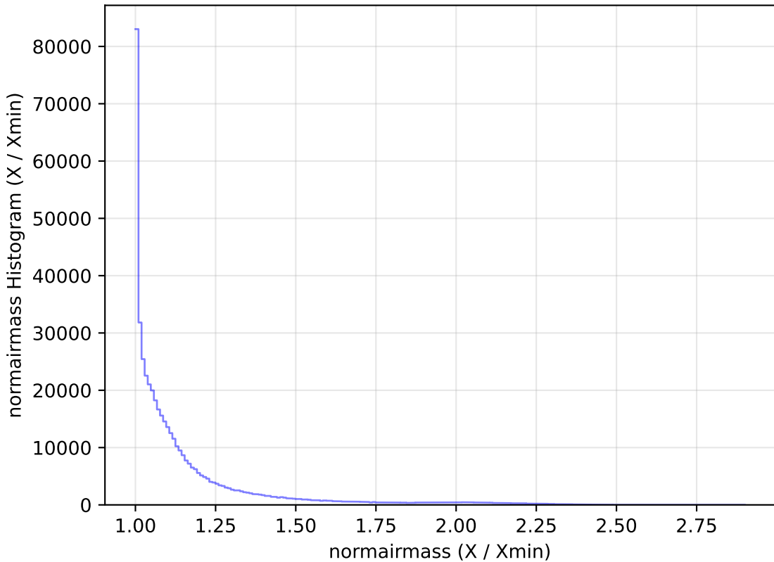
ddf_half_v3.4_10yrs All sky r band: normairmass Histogram
