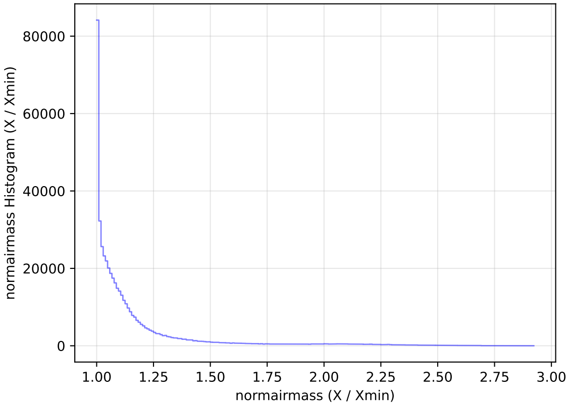
ddf_half_v3.4_10yrs All sky i band: normairmass Histogram
