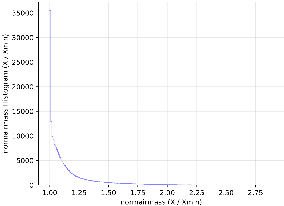
ddf_half_v3.4_10yrs All sky g band: normairmass Histogram
