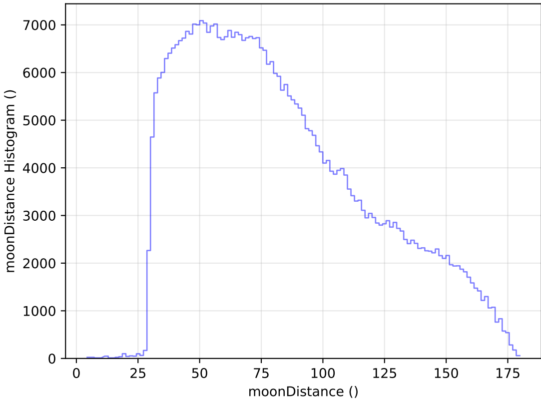
ddf_half_v3.4_10yrs WFD z band: moonDistance Histogram
