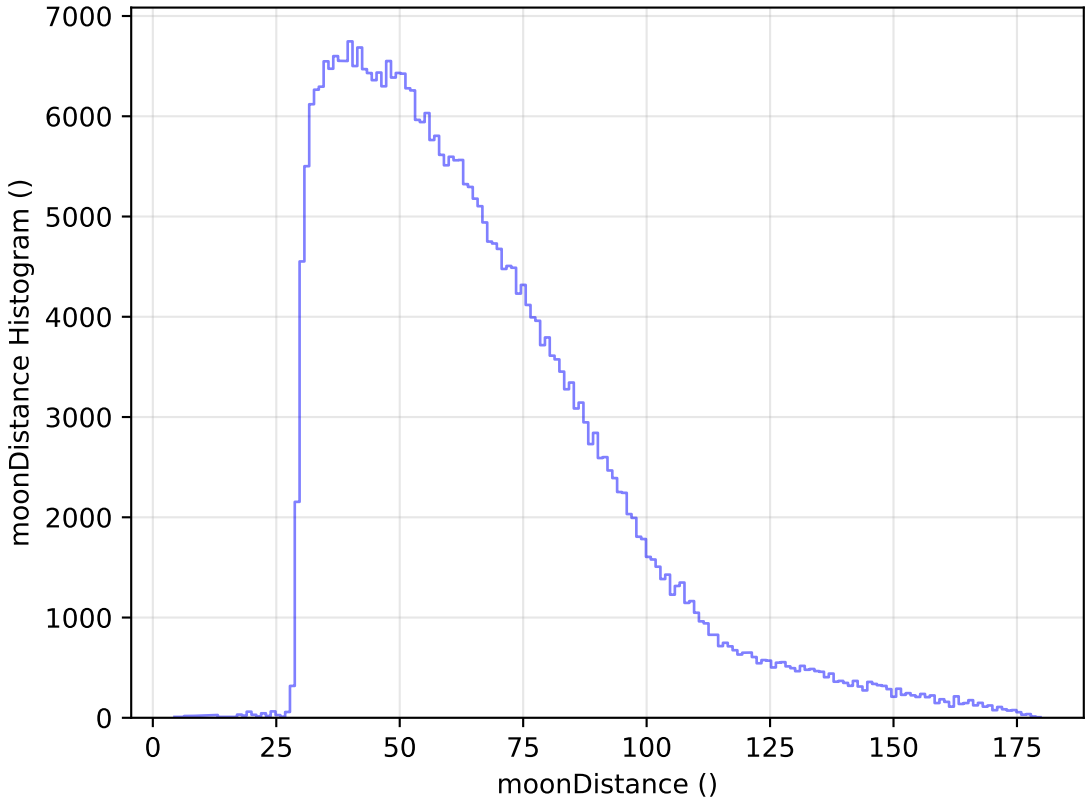
ddf_half_v3.4_10yrs WFD y band: moonDistance Histogram
