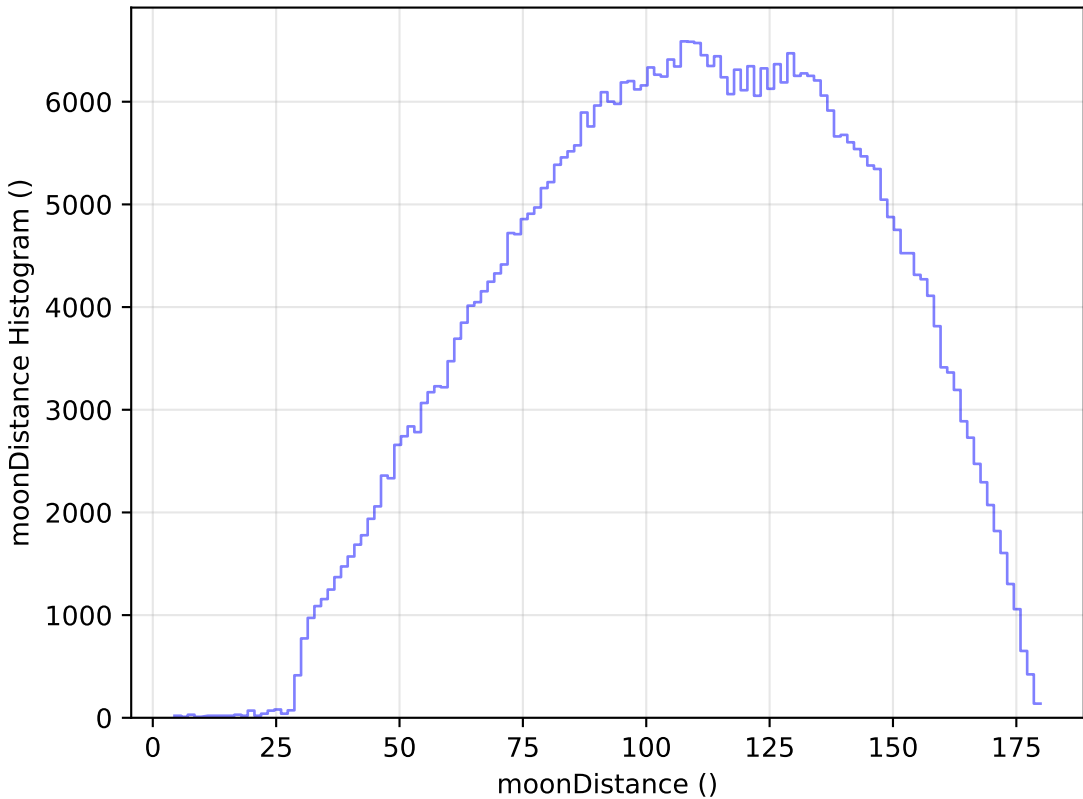
ddf_half_v3.4_10yrs WFD r band: moonDistance Histogram
