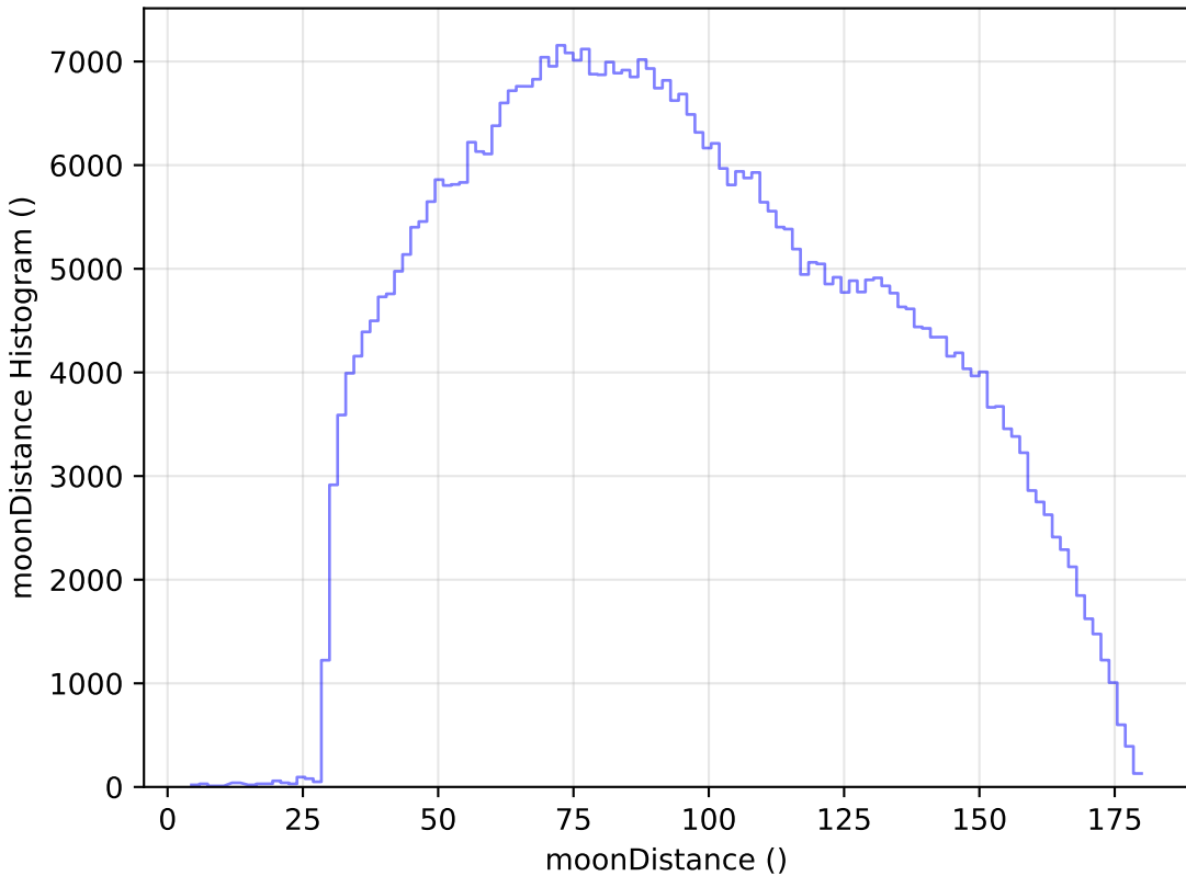
ddf_half_v3.4_10yrs WFD i band: moonDistance Histogram
