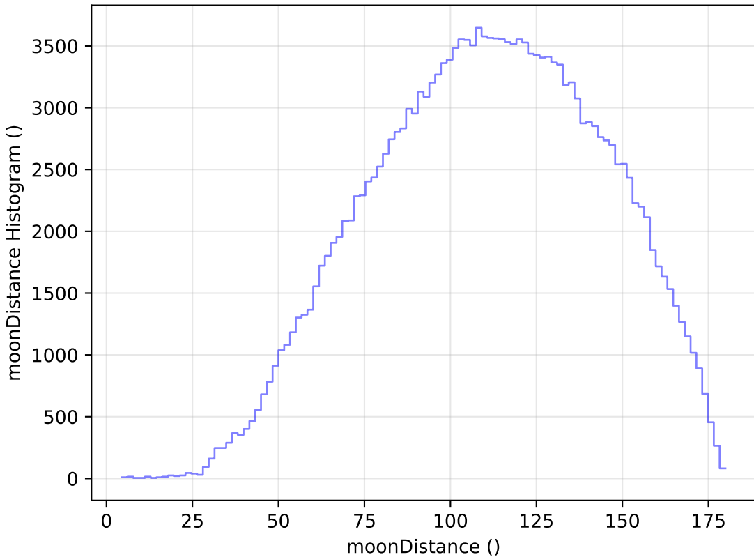
ddf_half_v3.4_10yrs WFD g band: moonDistance Histogram
