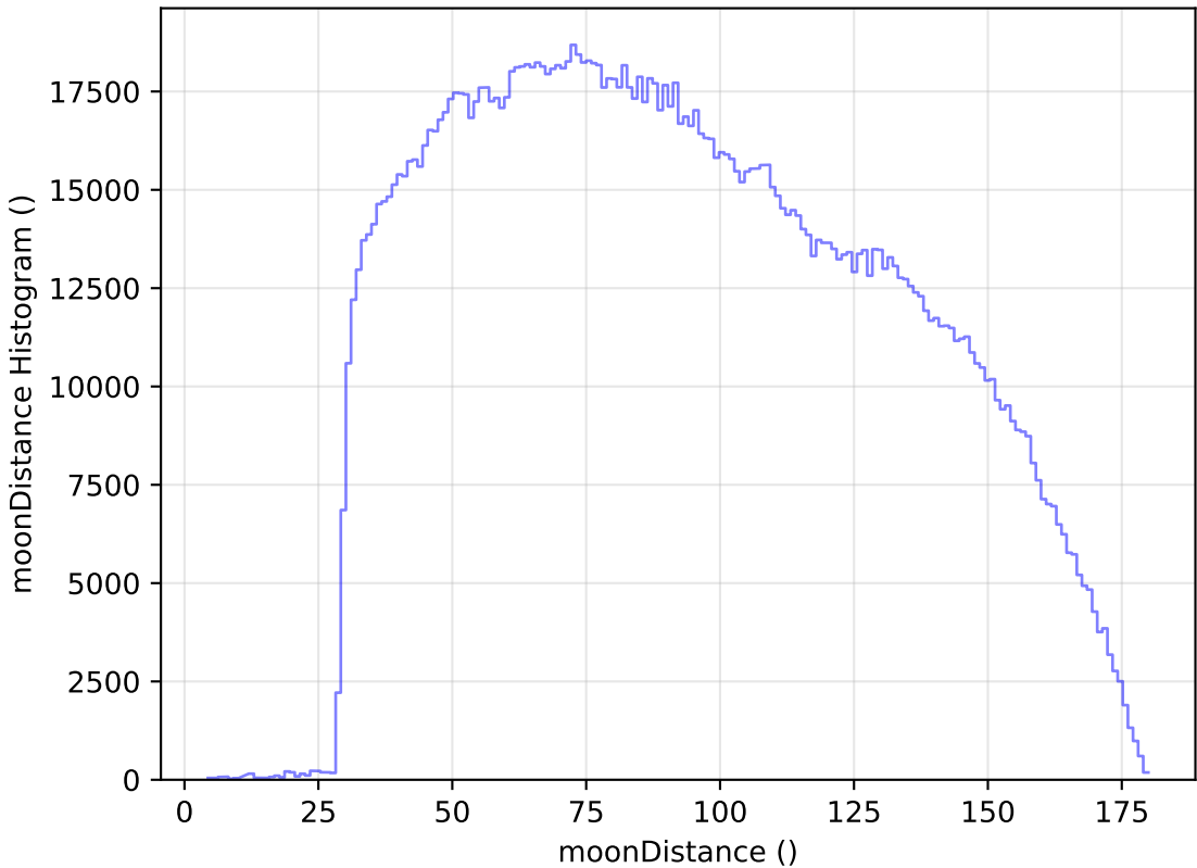
ddf_half_v3.4_10yrs WFD all bands: moonDistance Histogram
