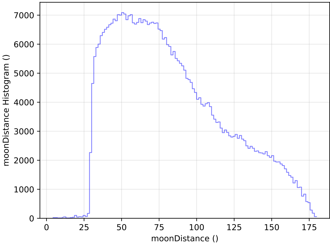
ddf_half_v3.4_10yrs All sky z band: moonDistance Histogram
