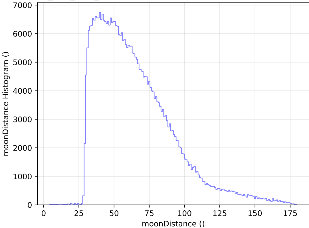
ddf_half_v3.4_10yrs All sky y band: moonDistance Histogram
