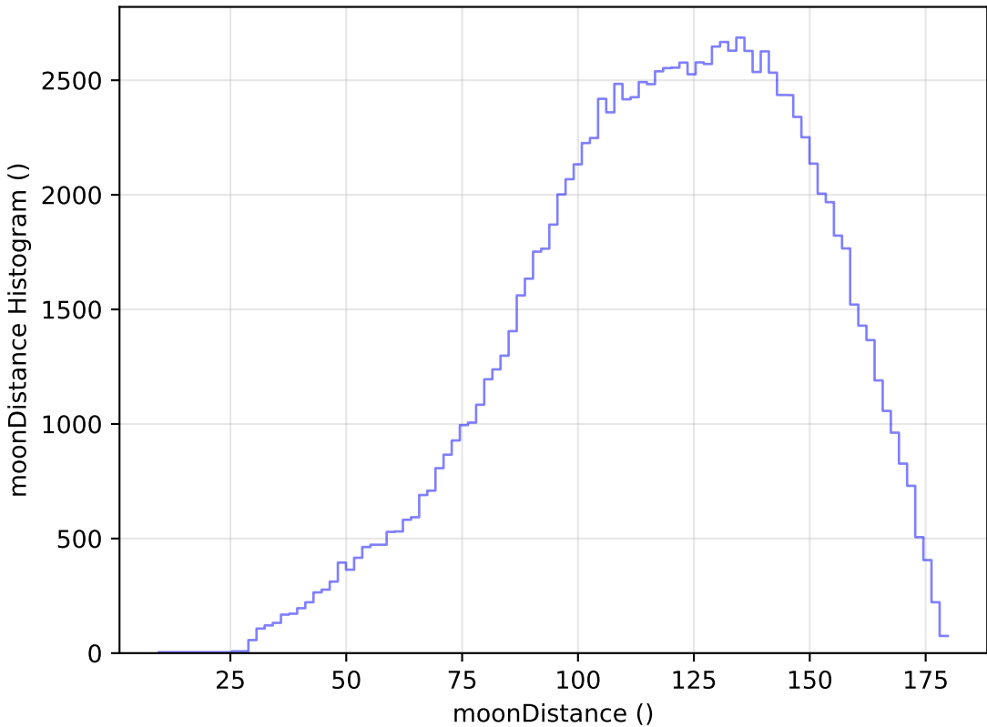
ddf_half_v3.4_10yrs All sky u band: moonDistance Histogram
