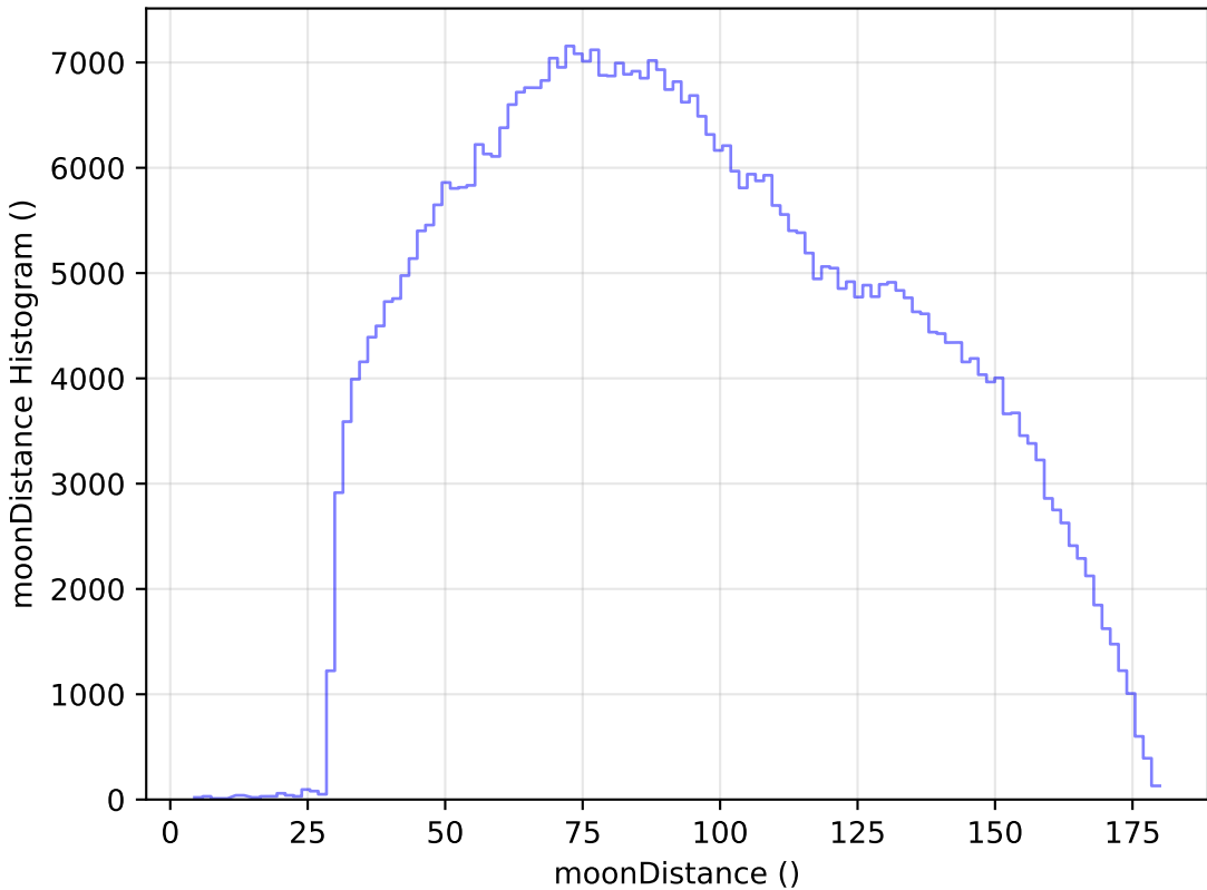
ddf_half_v3.4_10yrs All sky i band: moonDistance Histogram
