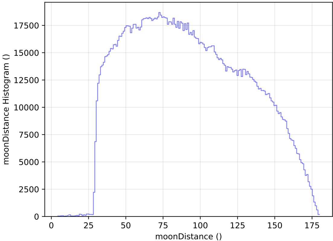
ddf_half_v3.4_10yrs All sky all bands: moonDistance Histogram
