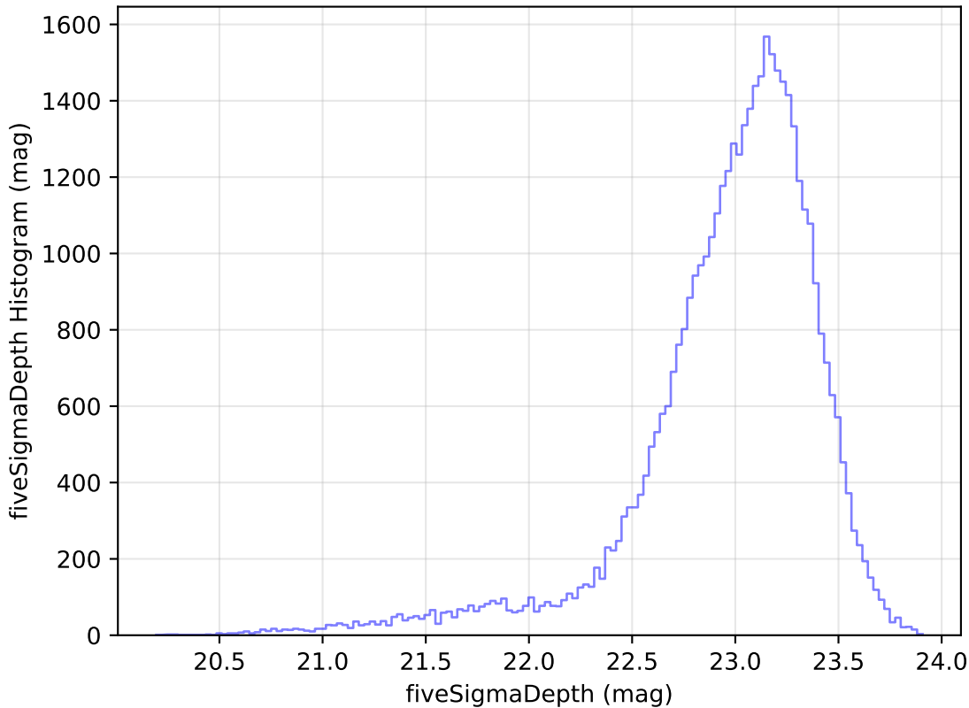
ddf_half_v3.4_10yrs Yr 1 z band: fiveSigmaDepth Histogram
