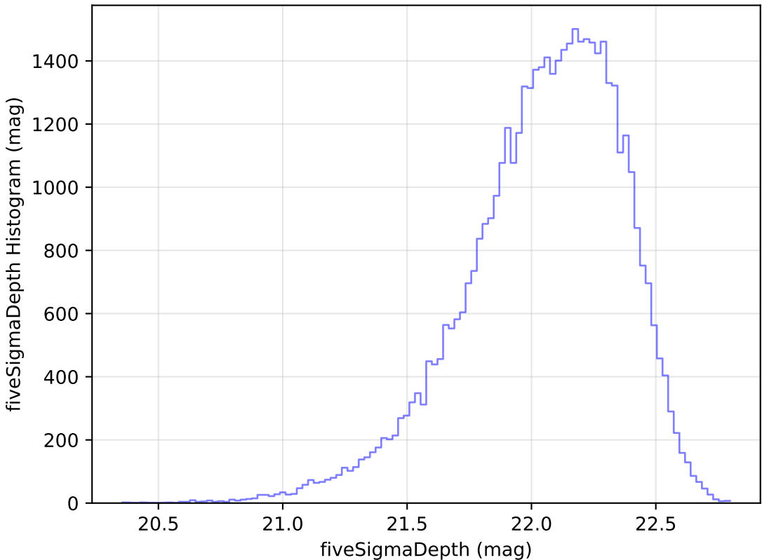
ddf_half_v3.4_10yrs Yr 1 y band: fiveSigmaDepth Histogram
