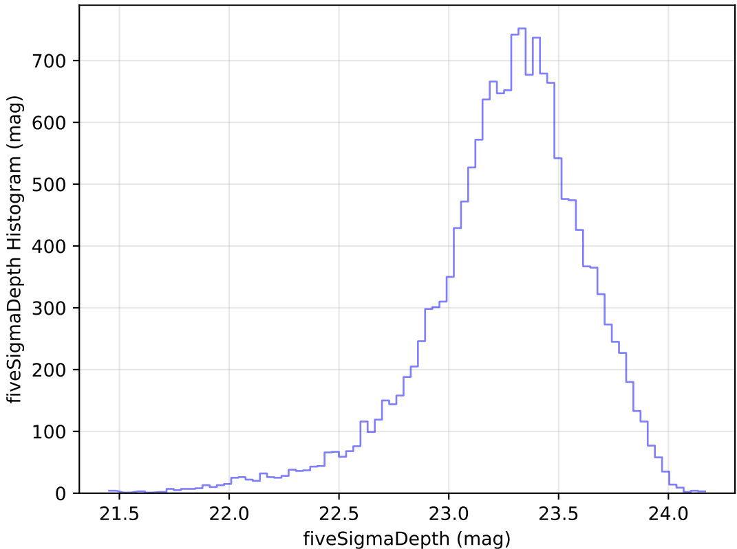
ddf_half_v3.4_10yrs Yr 1 u band: fiveSigmaDepth Histogram
