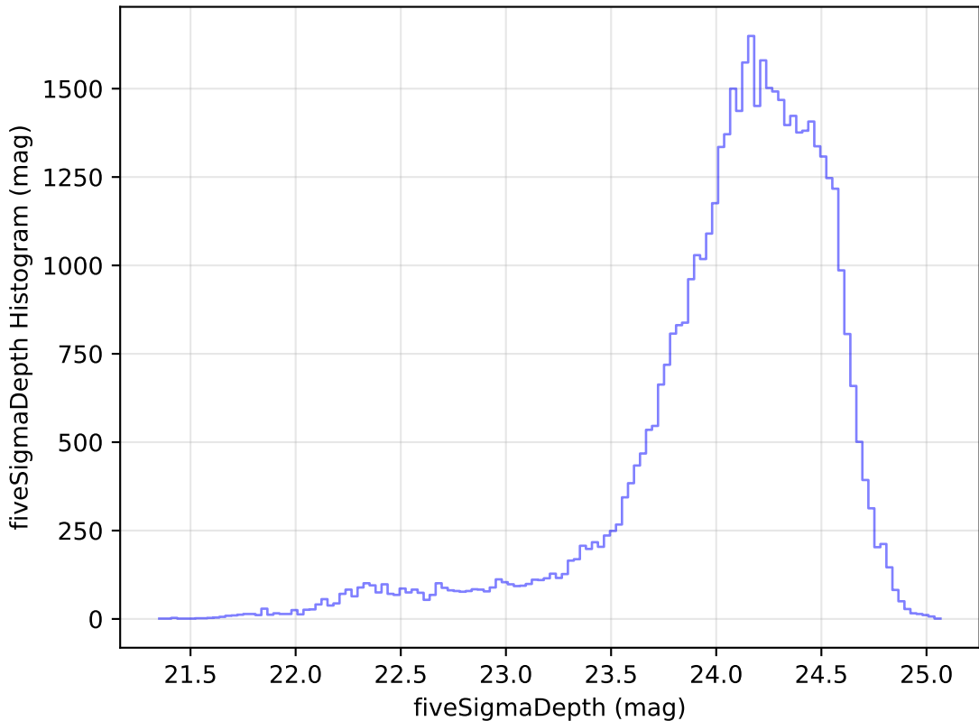
ddf_half_v3.4_10yrs Yr 1 r band: fiveSigmaDepth Histogram
