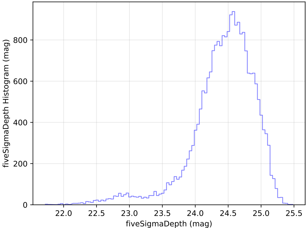
ddf_half_v3.4_10yrs Yr 1 g band: fiveSigmaDepth Histogram
