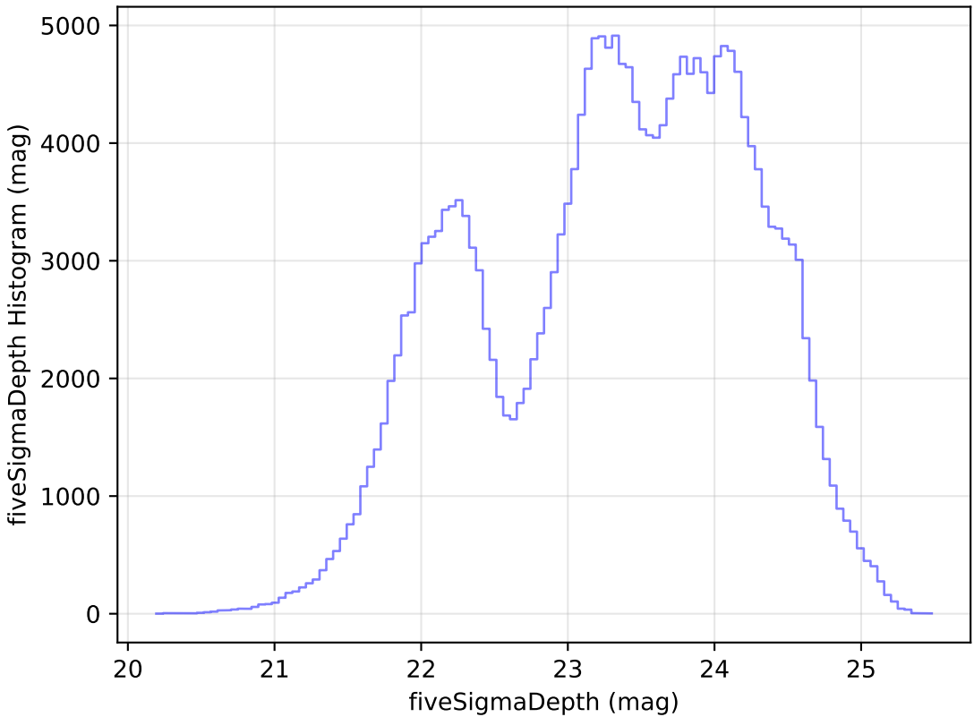
ddf_half_v3.4_10yrs Yr 1 all bands: fiveSigmaDepth Histogram
