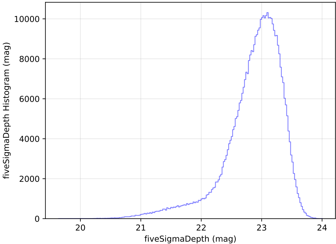
ddf_half_v3.4_10yrs WFD z band: fiveSigmaDepth Histogram
