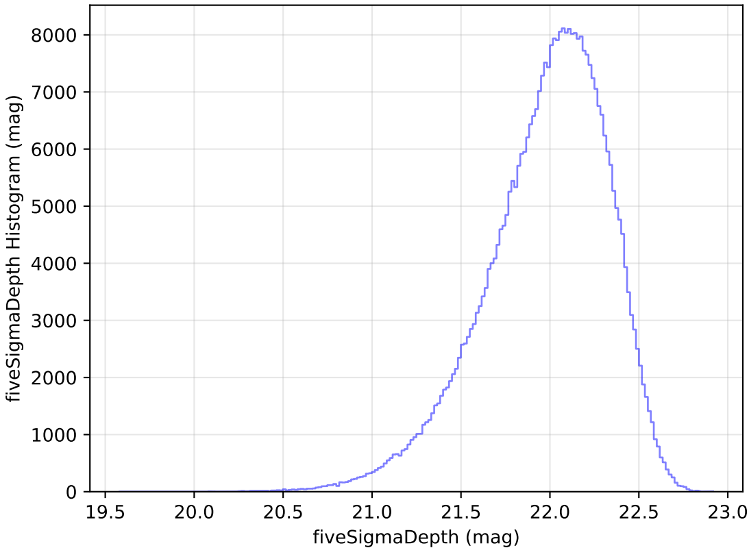
ddf_half_v3.4_10yrs WFD y band: fiveSigmaDepth Histogram
