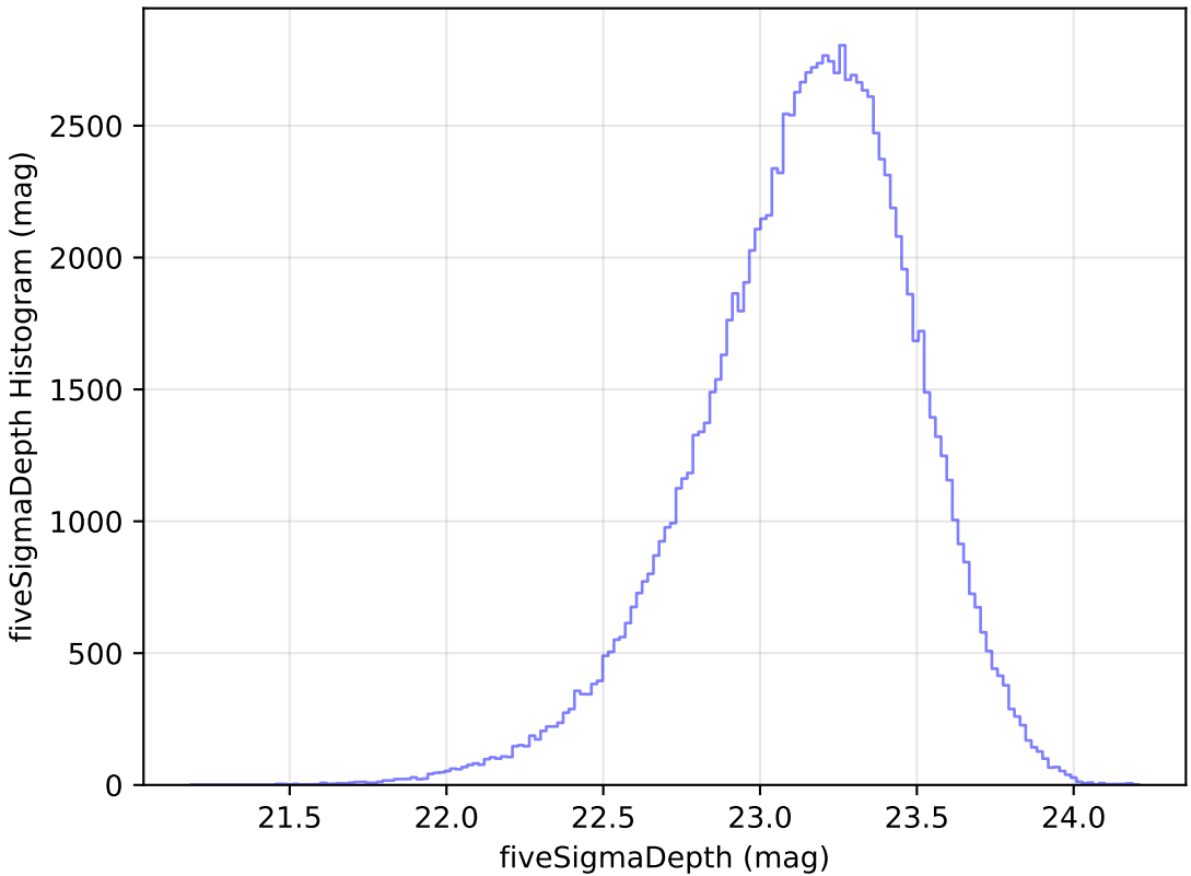
ddf_half_v3.4_10yrs WFD u band: fiveSigmaDepth Histogram
