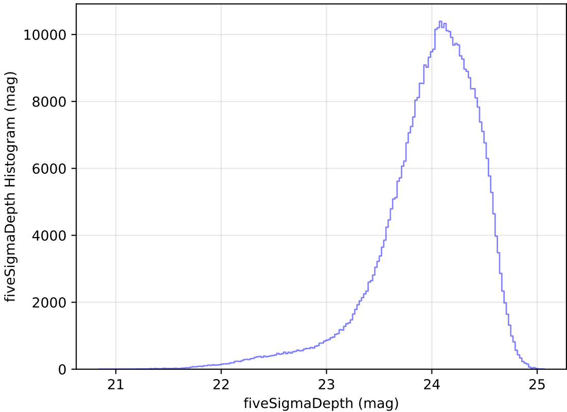
ddf_half_v3.4_10yrs WFD r band: fiveSigmaDepth Histogram
