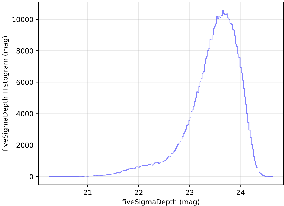
ddf_half_v3.4_10yrs WFD i band: fiveSigmaDepth Histogram
