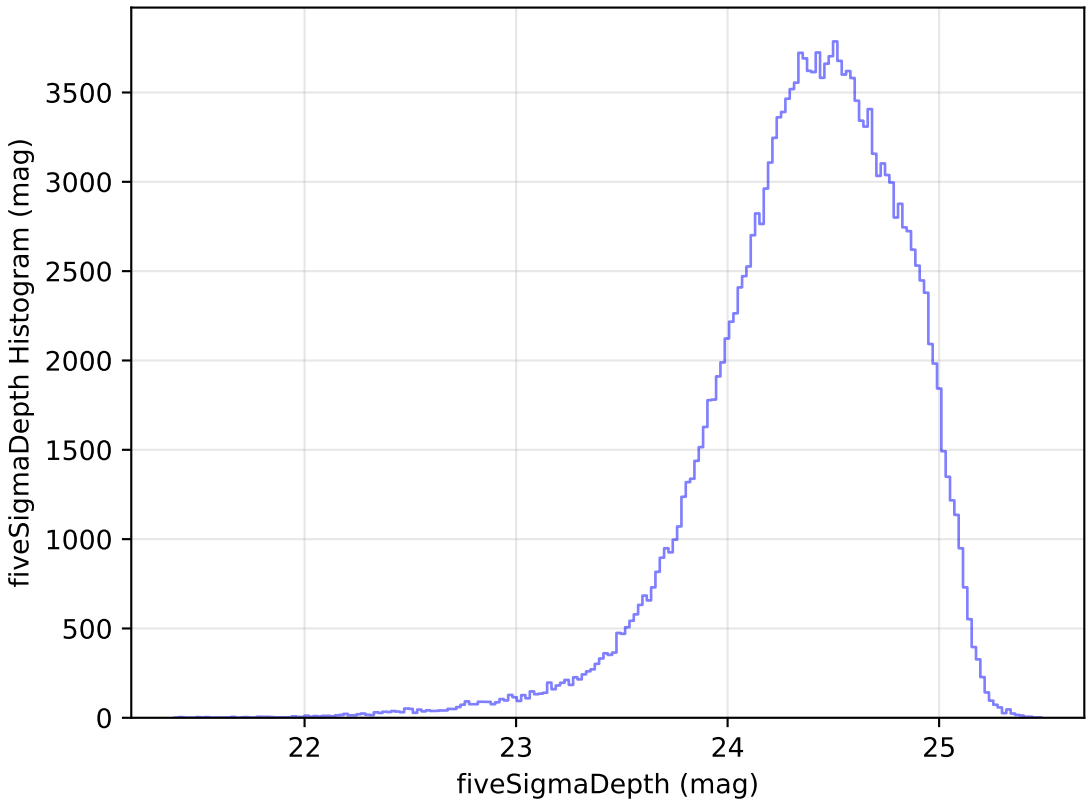
ddf_half_v3.4_10yrs WFD g band: fiveSigmaDepth Histogram
