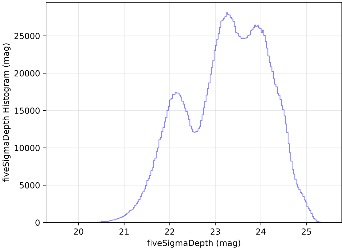
ddf_half_v3.4_10yrs WFD all bands: fiveSigmaDepth Histogram
