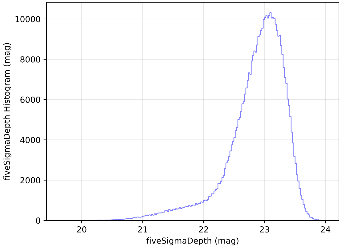
ddf_half_v3.4_10yrs All sky z band: fiveSigmaDepth Histogram
