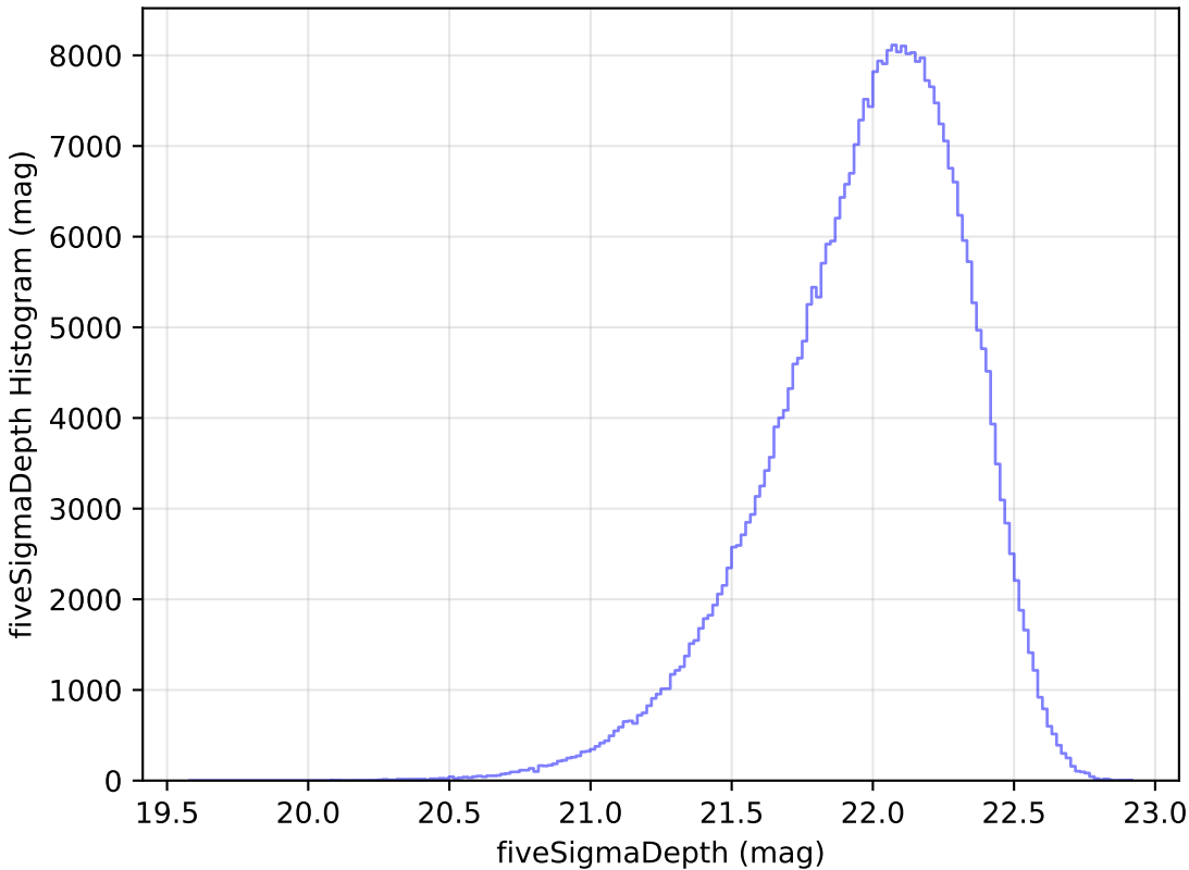
ddf_half_v3.4_10yrs All sky y band: fiveSigmaDepth Histogram
