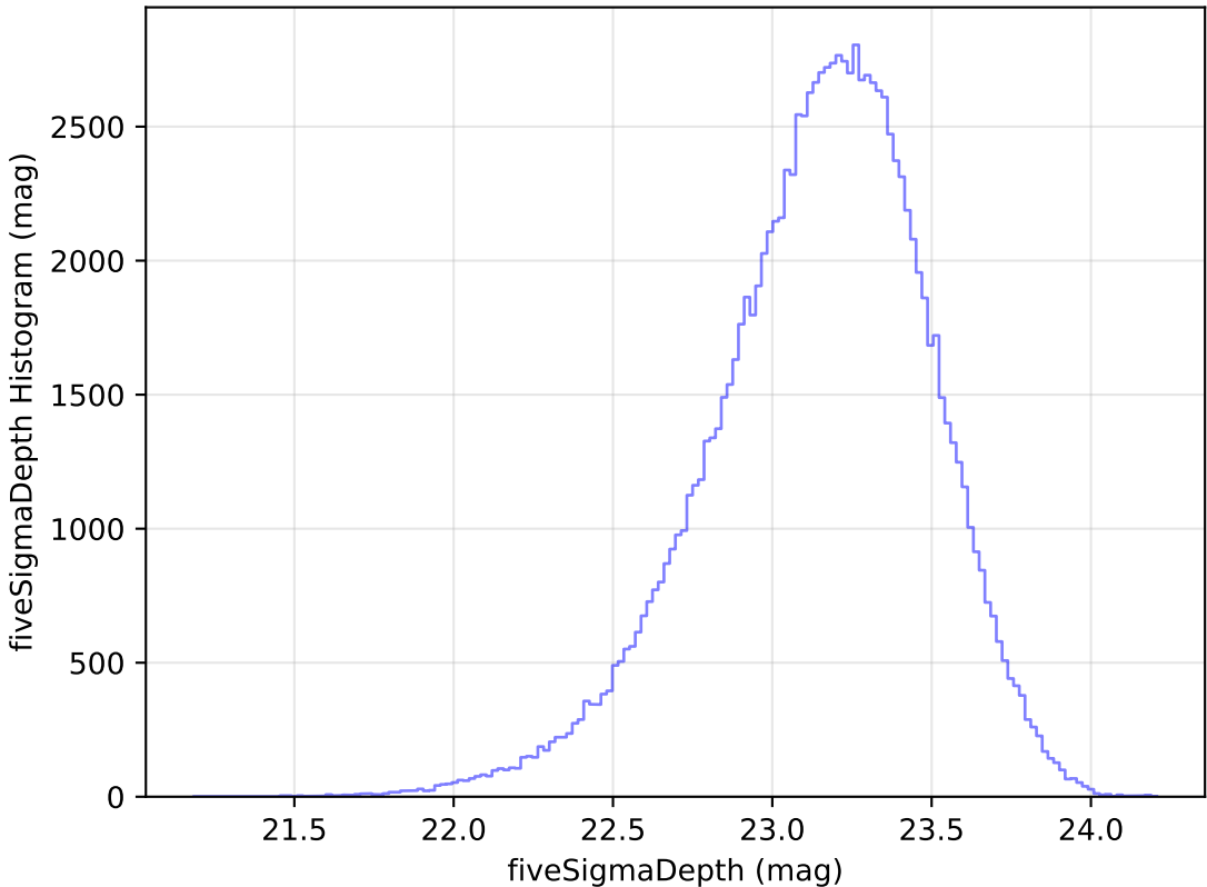
ddf_half_v3.4_10yrs All sky u band: fiveSigmaDepth Histogram
