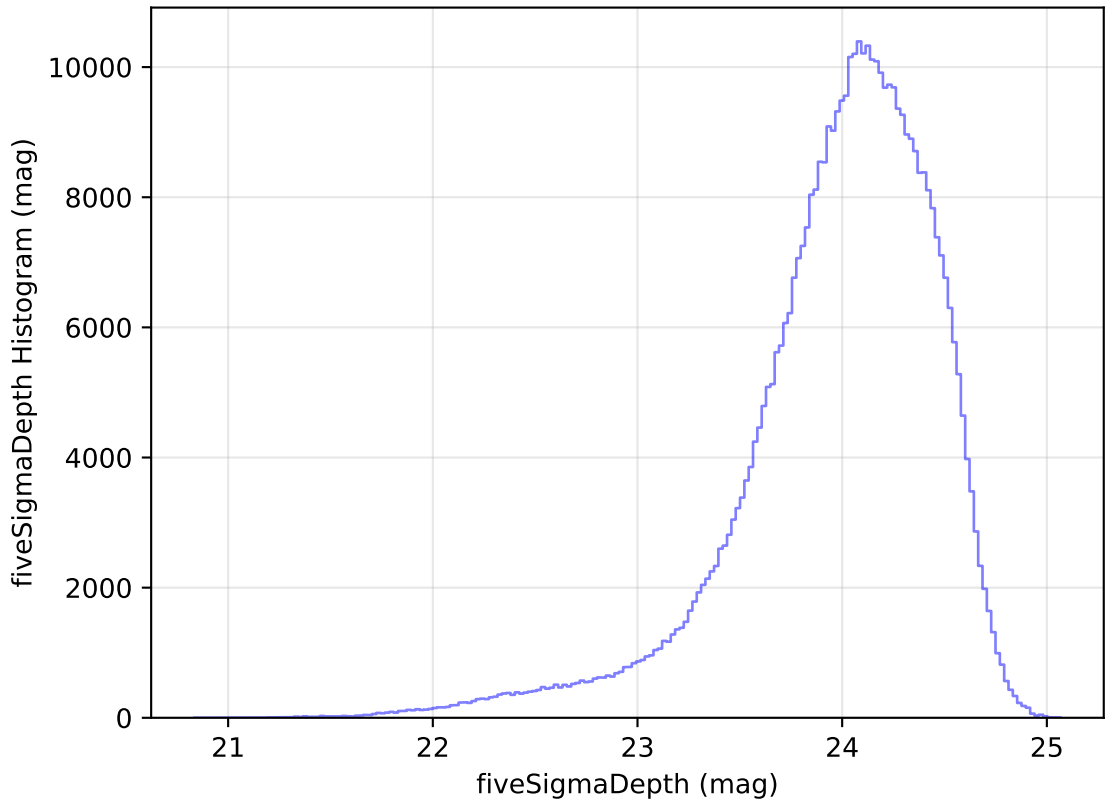
ddf_half_v3.4_10yrs All sky r band: fiveSigmaDepth Histogram
