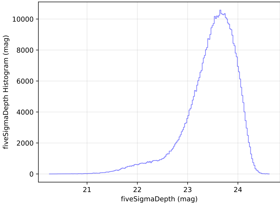
ddf_half_v3.4_10yrs All sky i band: fiveSigmaDepth Histogram
