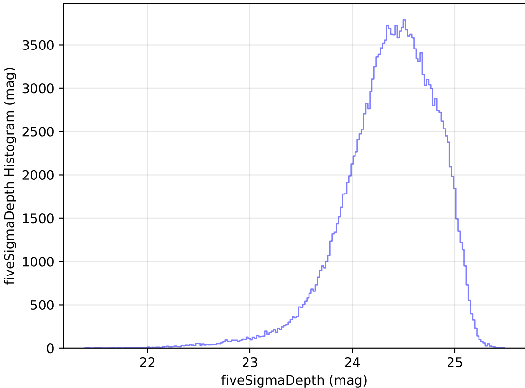
ddf_half_v3.4_10yrs All sky g band: fiveSigmaDepth Histogram
