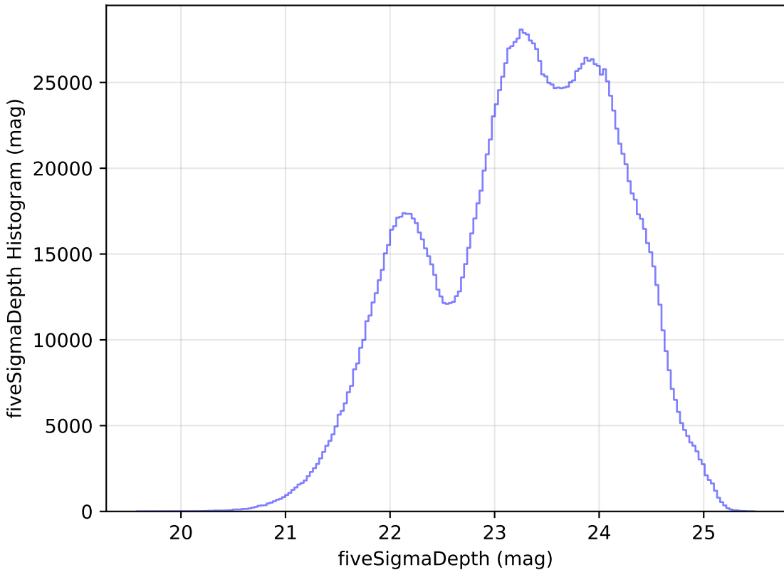
ddf_half_v3.4_10yrs All sky all bands: fiveSigmaDepth Histogram
