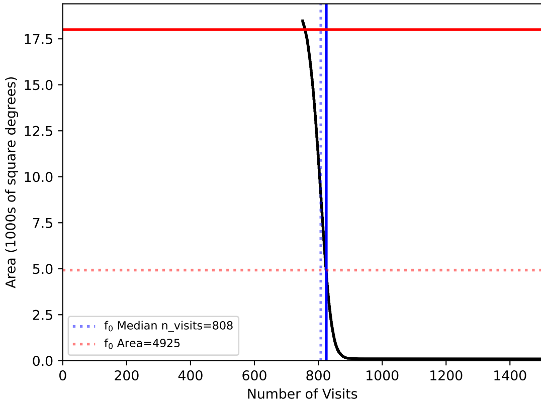
ddf_half_v3.4_10yrs WFD: f0
