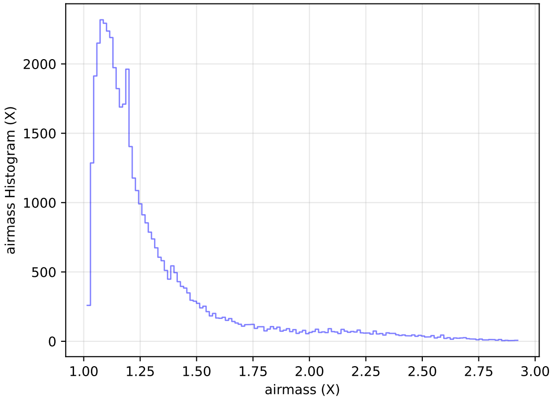
ddf_half_v3.4_10yrs Yr 1 z band: airmass Histogram
