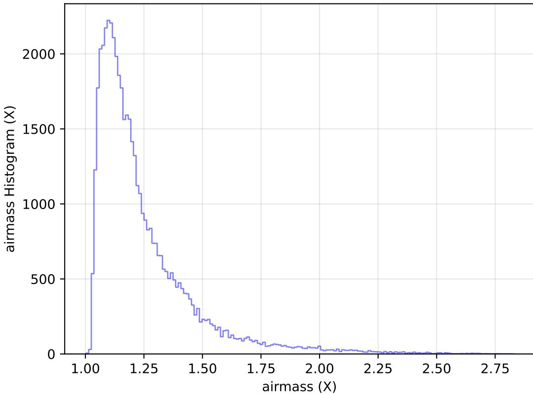
ddf_half_v3.4_10yrs Yr 1 y band: airmass Histogram
