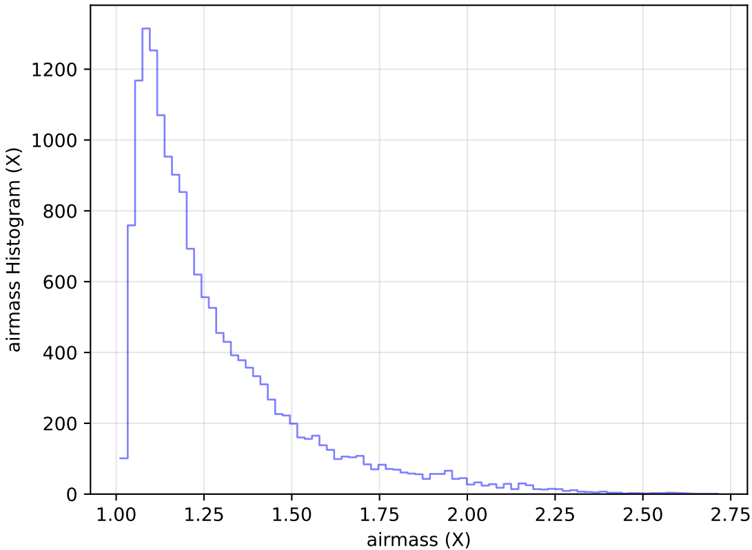
ddf_half_v3.4_10yrs Yr 1 u band: airmass Histogram
