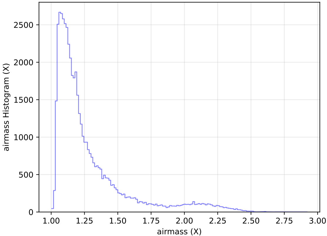
ddf_half_v3.4_10yrs Yr 1 r band: airmass Histogram
