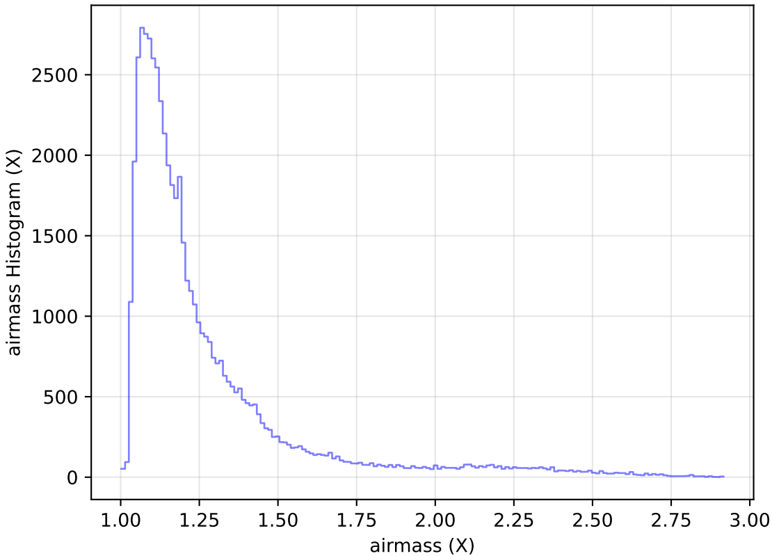
ddf_half_v3.4_10yrs Yr 1 i band: airmass Histogram
