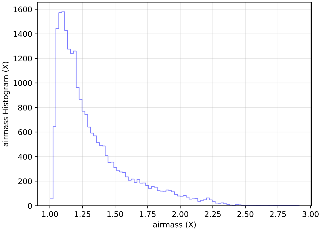
ddf_half_v3.4_10yrs Yr 1 g band: airmass Histogram
