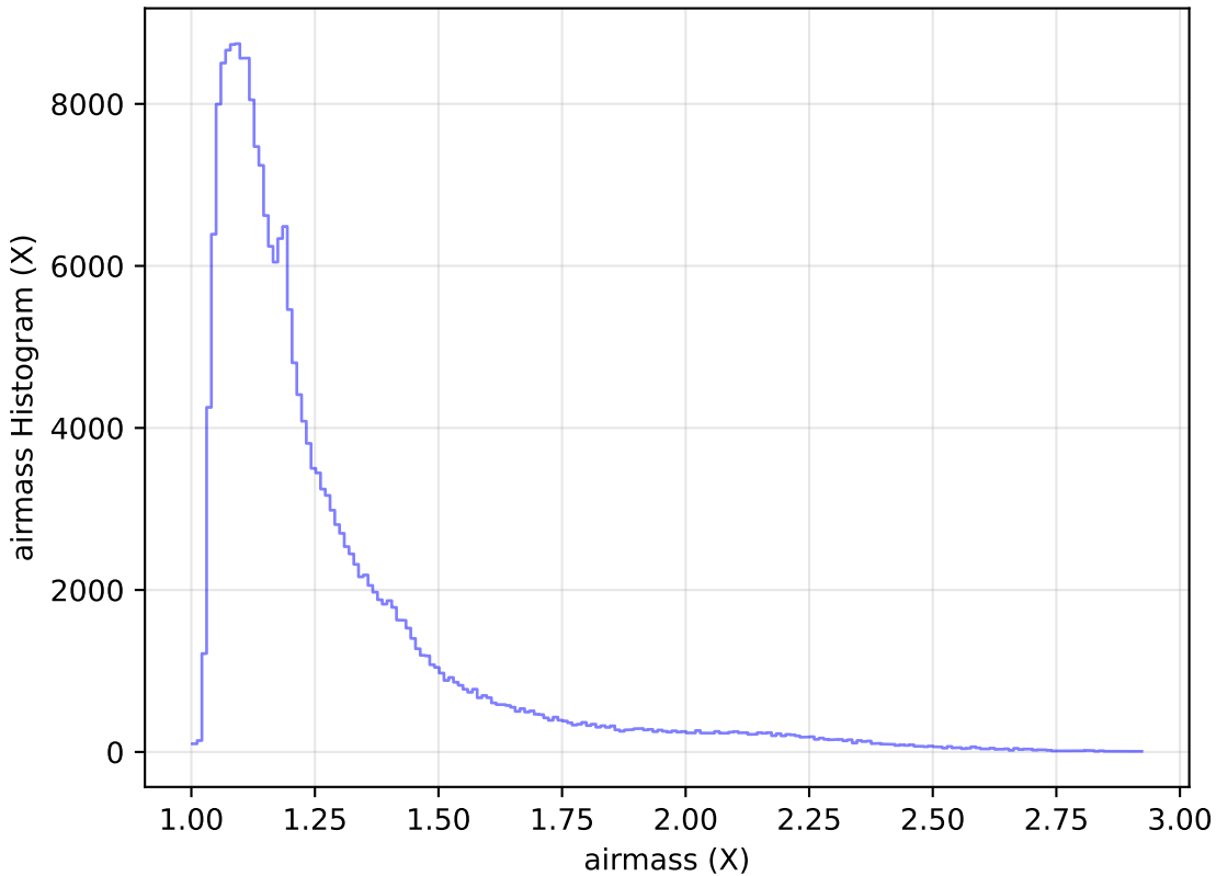
ddf_half_v3.4_10yrs Yr 1 all bands: airmass Histogram
