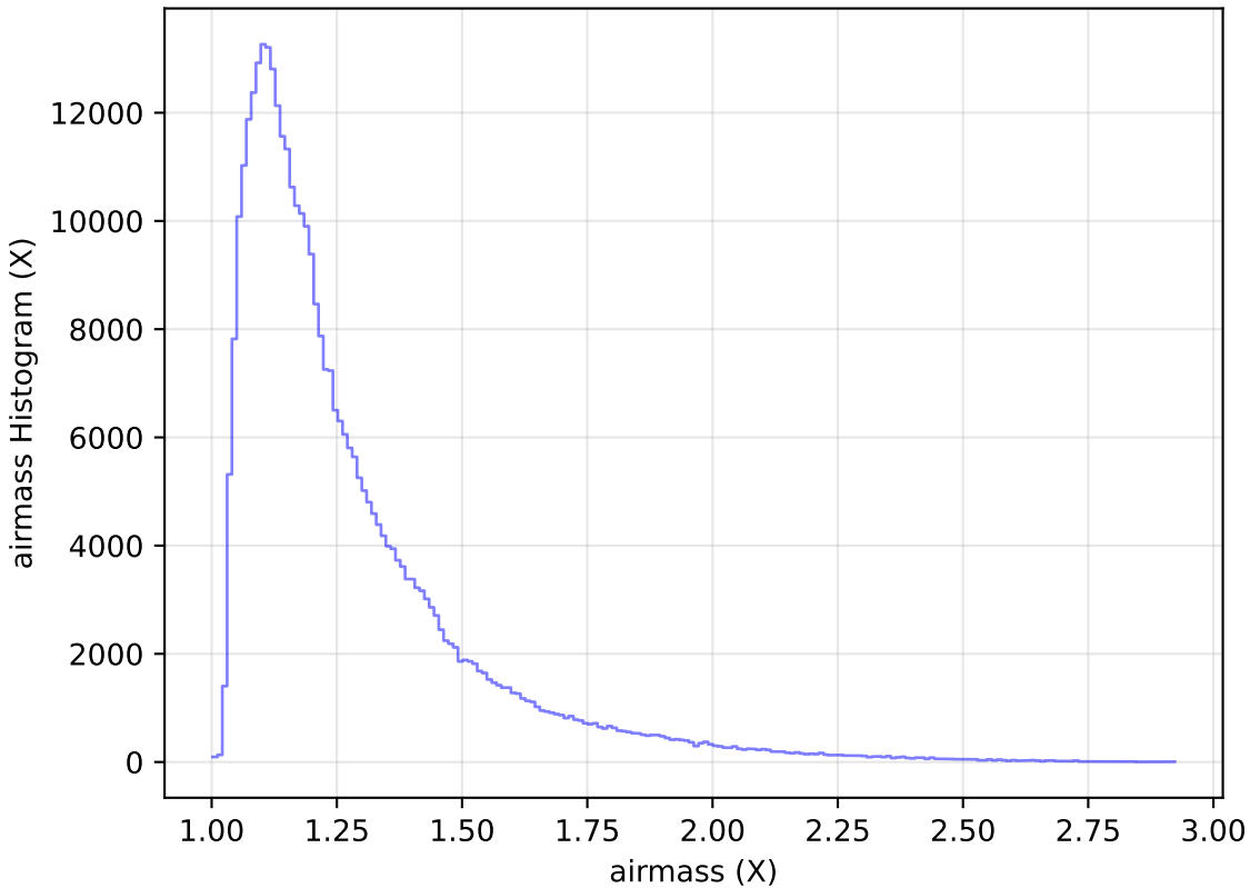
ddf_half_v3.4_10yrs WFD y band: airmass Histogram
