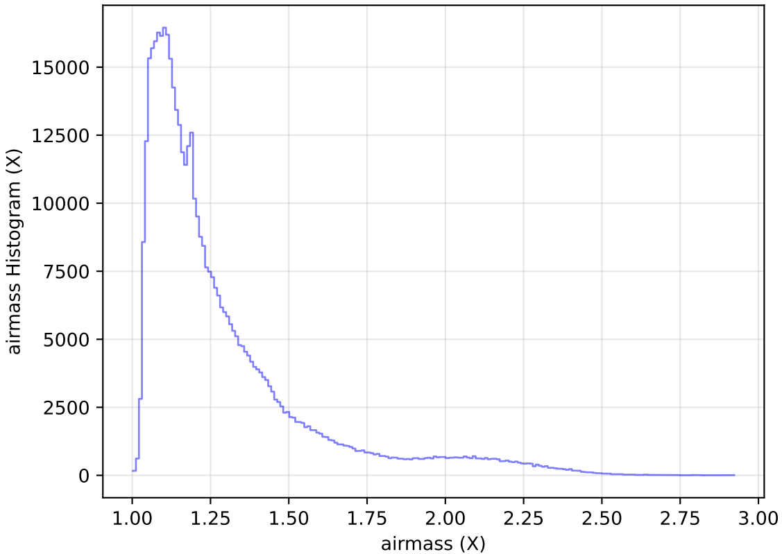
ddf_half_v3.4_10yrs WFD r band: airmass Histogram
