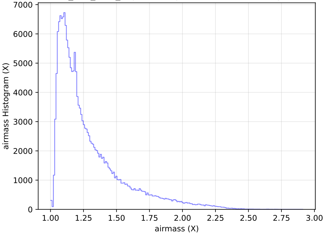
ddf_half_v3.4_10yrs WFD g band: airmass Histogram
