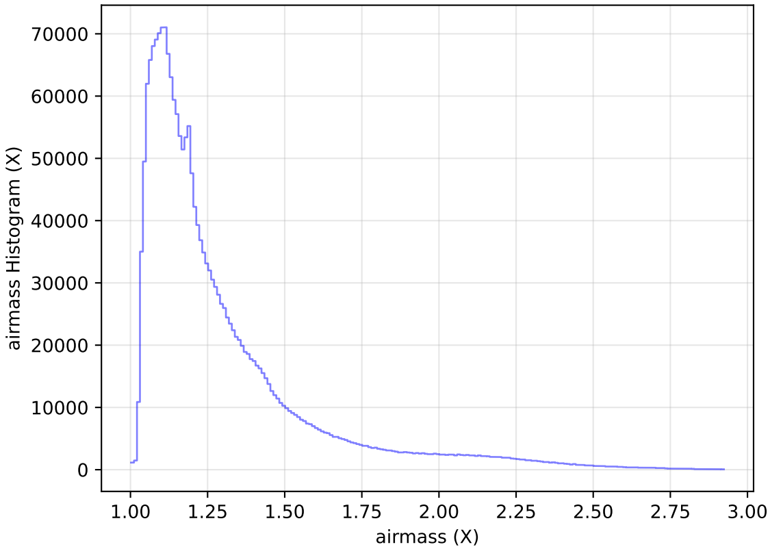
ddf_half_v3.4_10yrs WFD all bands: airmass Histogram
