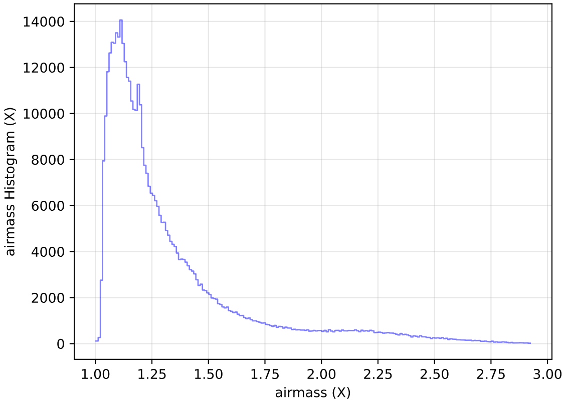
ddf_half_v3.4_10yrs All sky z band: airmass Histogram
