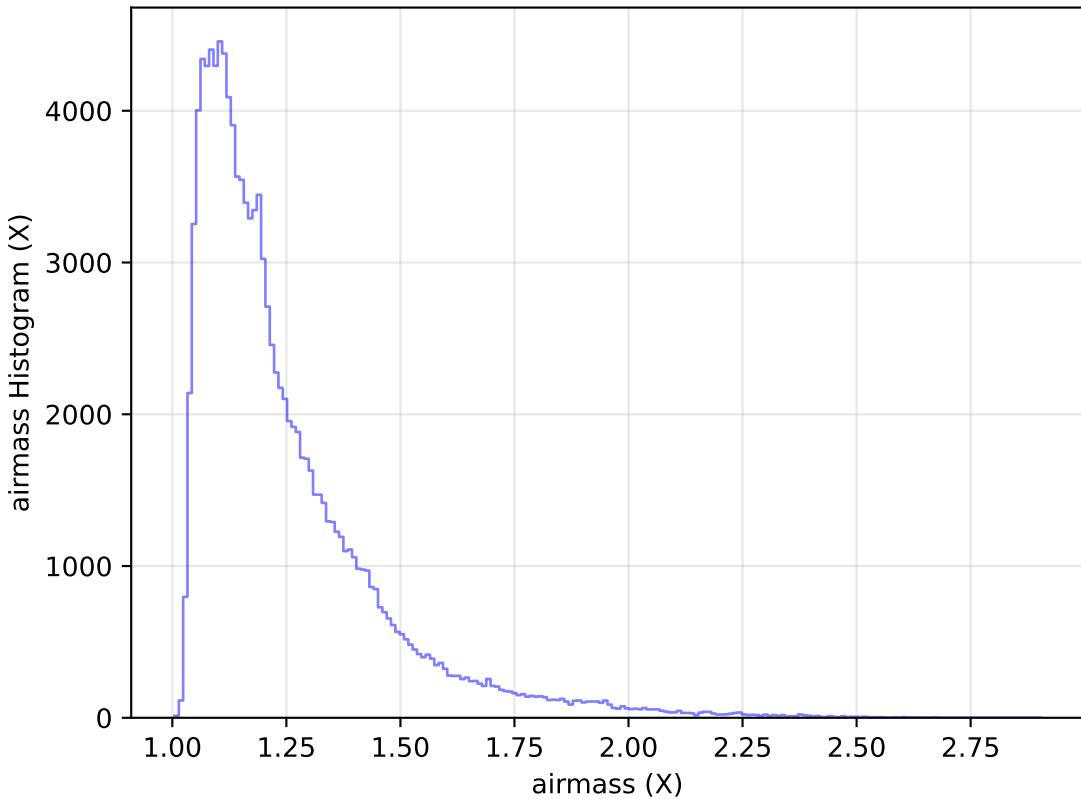
ddf_half_v3.4_10yrs All sky u band: airmass Histogram
