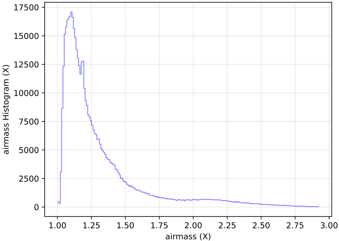
ddf_half_v3.4_10yrs All sky i band: airmass Histogram
